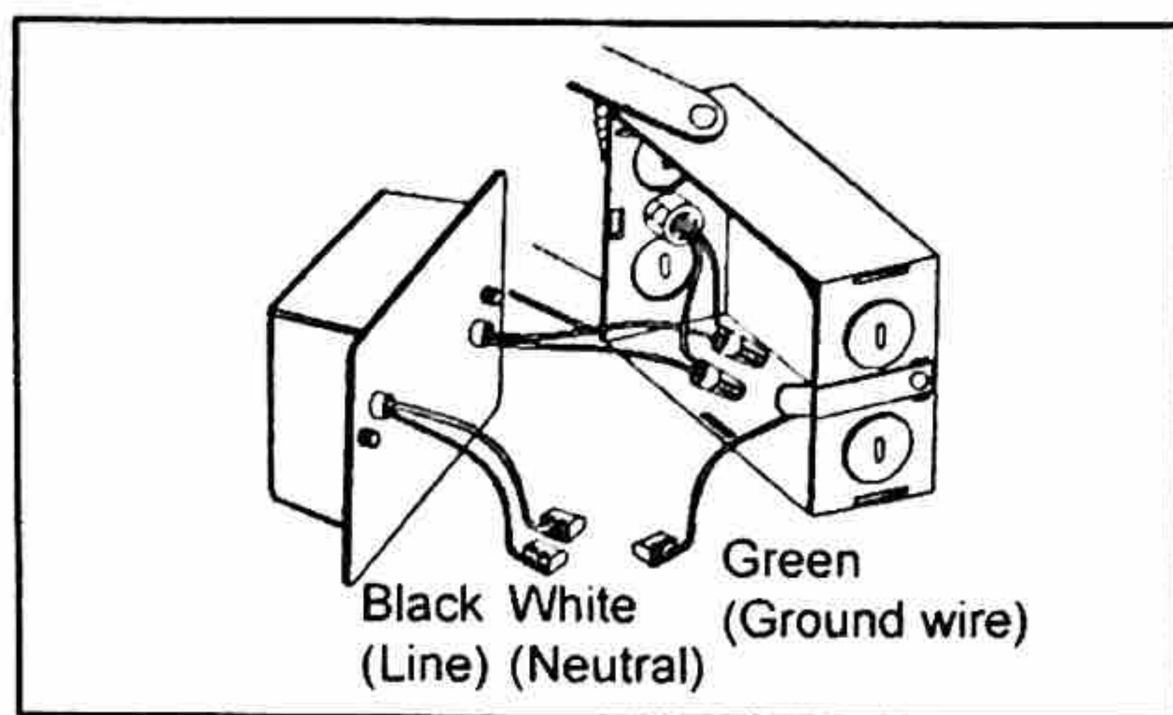
120V J-Box
