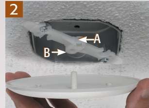
Use the opening in the bracket most suitable for your ceiling condition... 'A' for flat ceilings, push post into opening to seat cover; 'B' for uneven or textured ceilings, screw threaded post into opening until tight.
