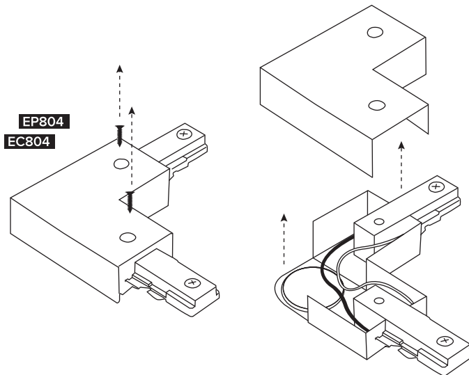
STEP 1. Unscrew (2) screws and removed top L-shaped cover.
