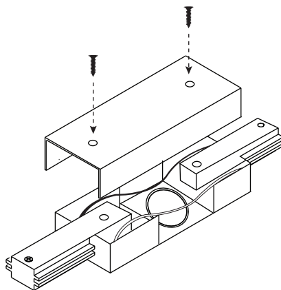
STEP 3. Screw straight shaped cover included
