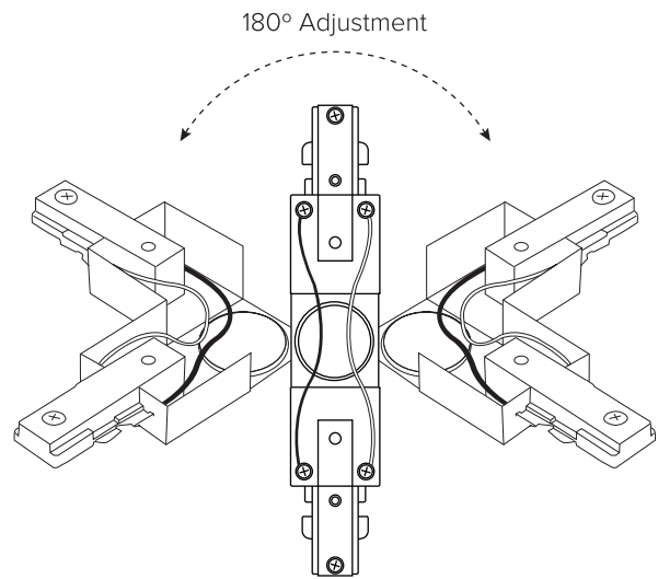
STEP 2. Manually adjust connector until is fully straight.
