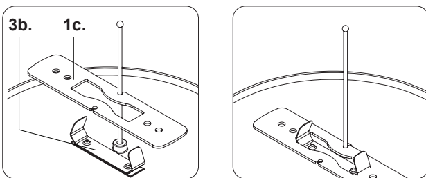
Illustration 2: Attaching to the mounting plate
