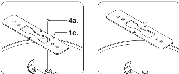
Illustration 1: Attaching safety cable
