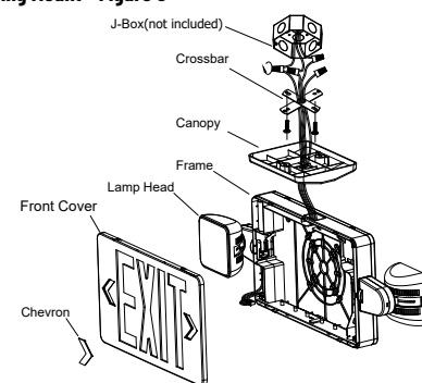
Ceiling Mount - Figure 3
