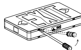
Wall Mount - Figure 2
