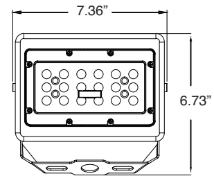
29W Yoke (Dedicated CCT)
