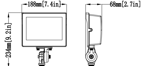
15-25W 1/2" Threaded Knuckle (CCT Selectable)
