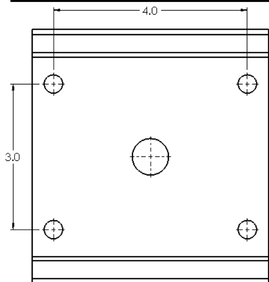
WALL MOUNT DETAIL
