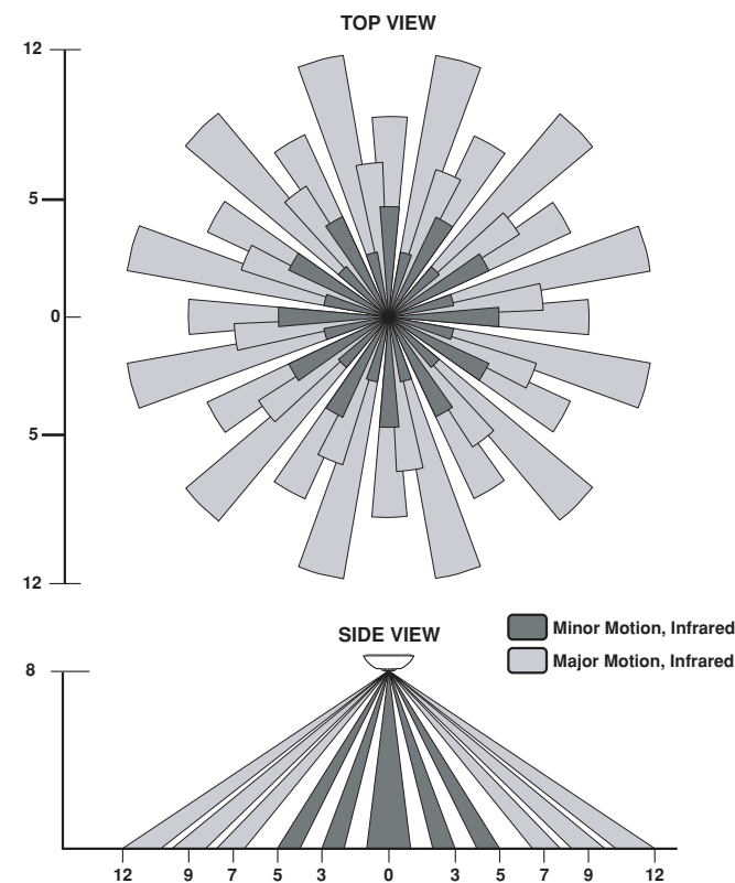
Figure 2 (Cat. No. OSC04) Field-of-View Ranges
