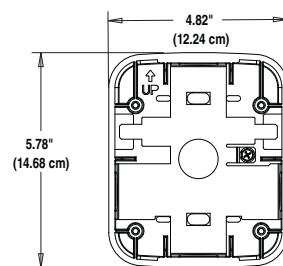
Surface Mount Back Box for Walls ( SBBRL/SBBWL)
