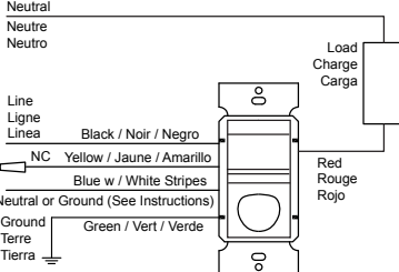
Figure 4: Single Pole Configuration
