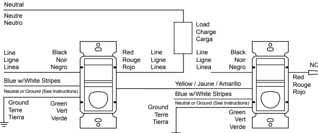
Figure 6: Multilocation Configuration
