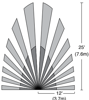
Figure 1: Sensor Coverage Area
