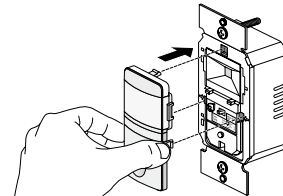
Figure 9: Replace Front Cover
