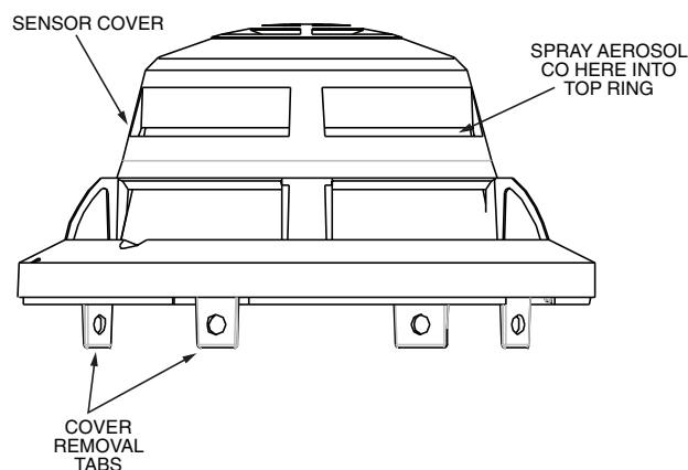
FIGURE 3. CO TESTING:
