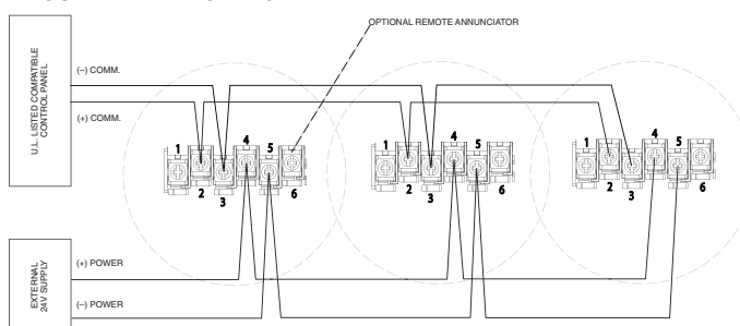
FIGURE 1. WIRING DIAGRAM:
