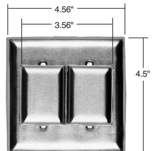
Dimensions for WP2
