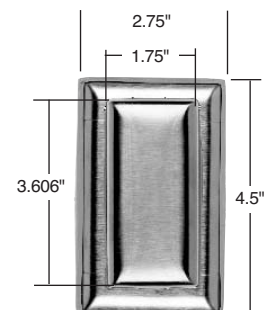
Dimensions for WP8 & WP26
