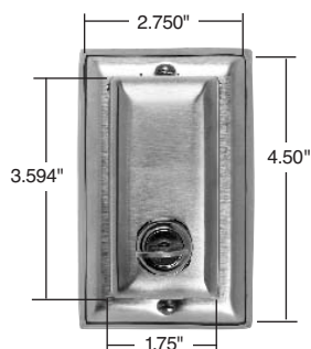
Dimensions for Vertical Locking
