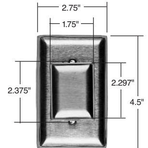
Dimensions for WP1 & WP7
