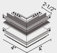
FG-RTL-ACC-4
