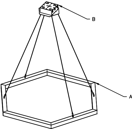
CUZTOM CANOPY DETAIL(CENTER OF FIXTURE)
