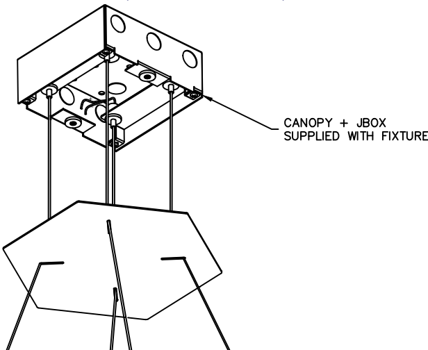
CUZTOM CANOPY DETAIL(CENTER OF FIXTURE)
